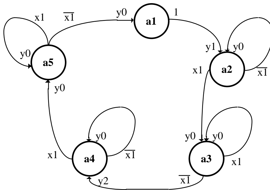
Transition table a(t+1)=\delta(a(t),x(t))
